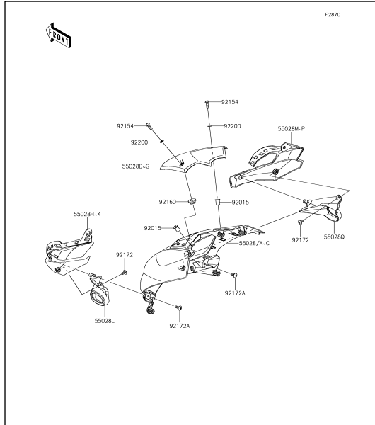
65 Cowling(Upper)
