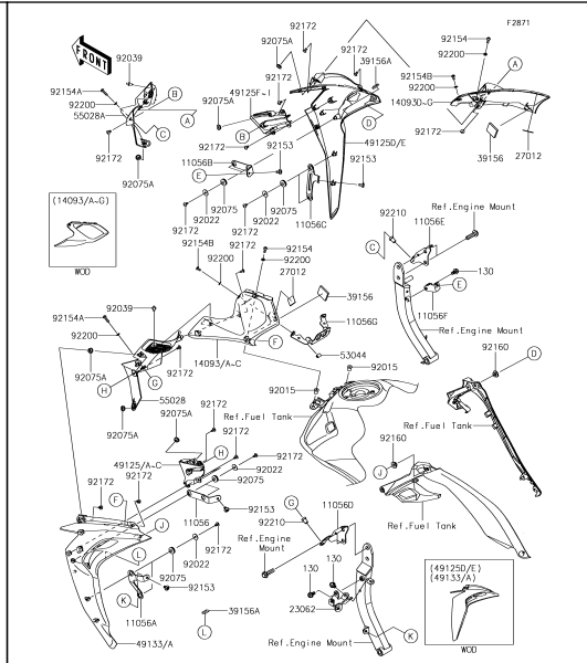
66 Cowling(Center)
