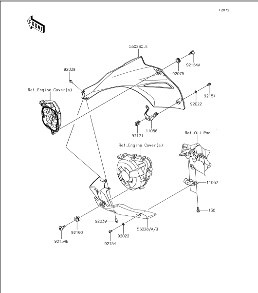
67 Cowling(Lowers)
