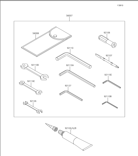
59 Owner's Tools
