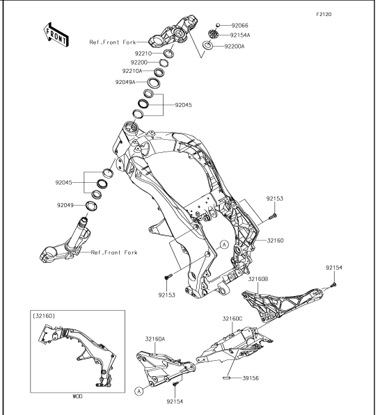
28 Frame
