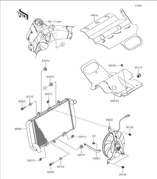
26 Radiator
