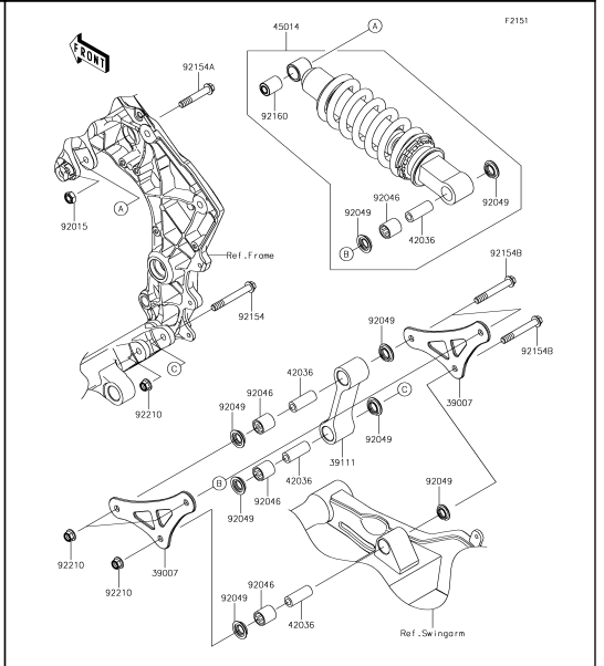
32 Suspension/Shock Absorber
