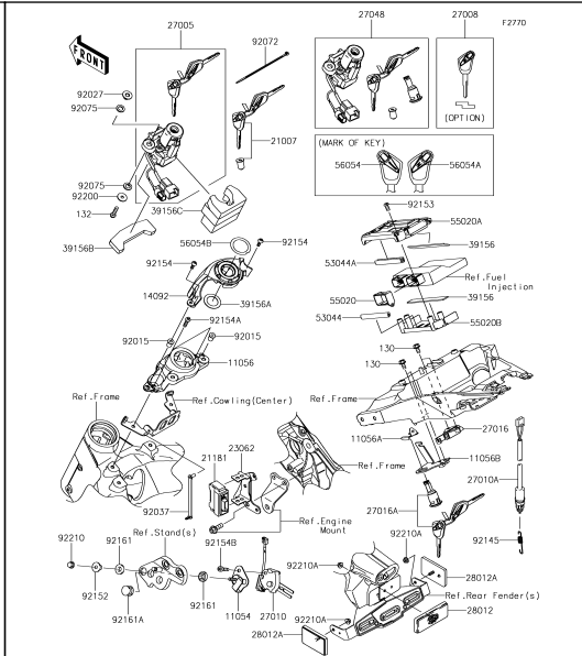
58 Ignition Switch
