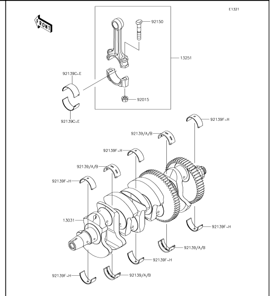
8 Crankshaft
