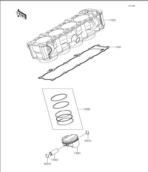
3 Cylinder/Piston(s)
