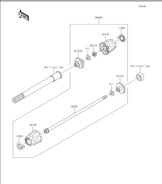
71 Accessory(Axle Slider)
