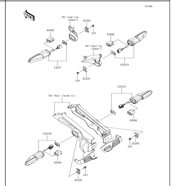
56 Turn Signals(HJF)
