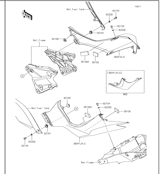
52 Side Covers
