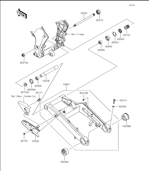
31 Swingarm
