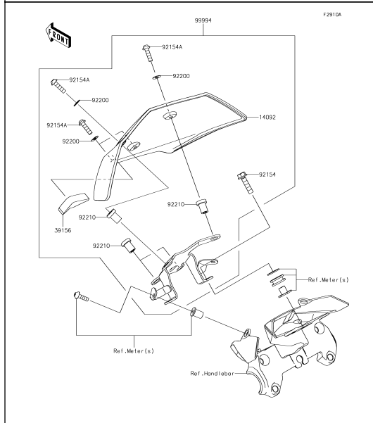
69 Accessory(Meter Cover)
