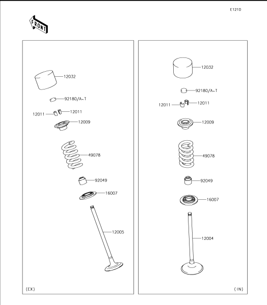
6 Valve(s)
