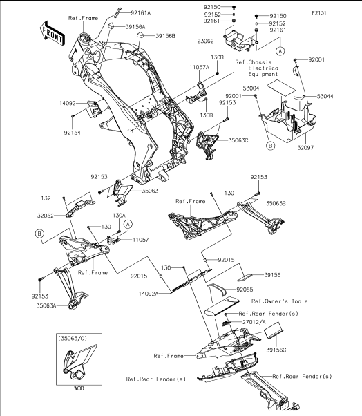
30 Frame Fittings
