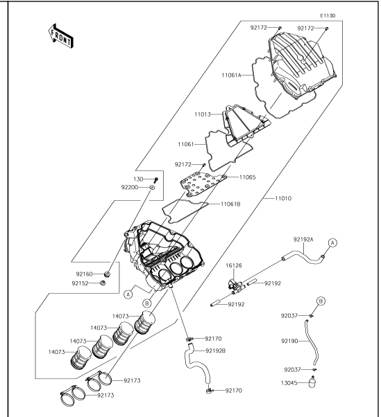
4 Air Cleaner
