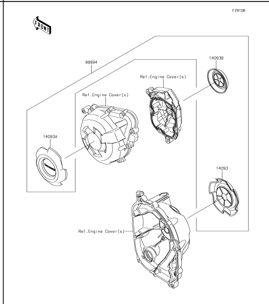
70 Accessory(Crankcase Ring)
