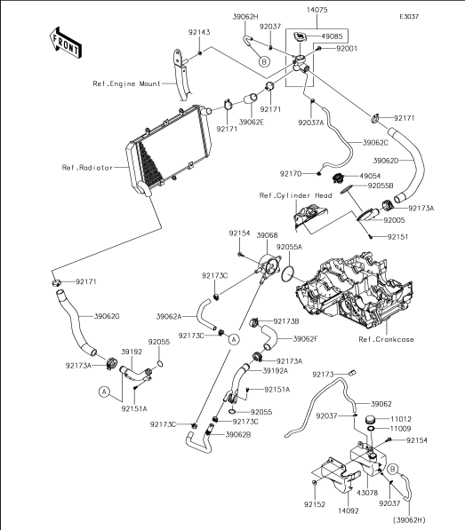
27 Water Pipe
