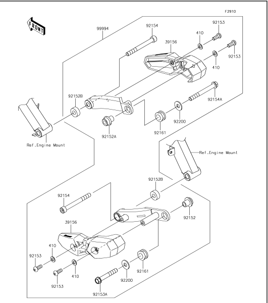
68 Accessory(Shroud Slider)
