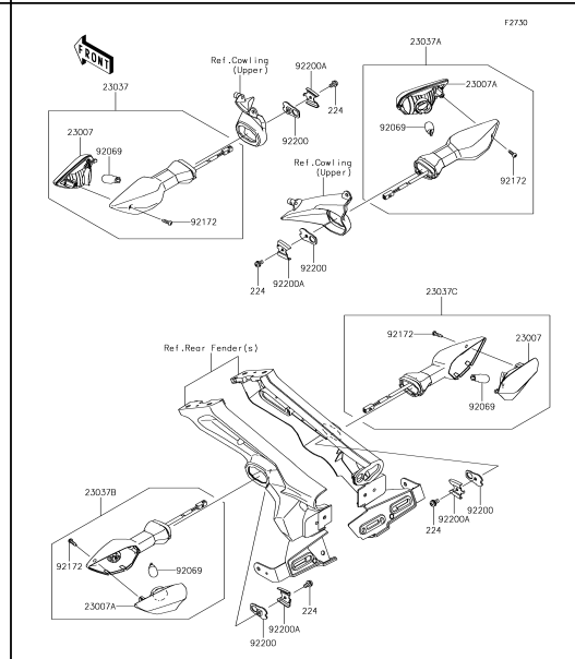
55 Turn Signals(HHF)
